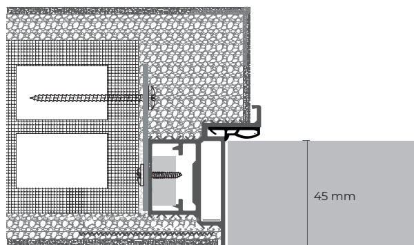
45 mm - a tirare 45 mm - pull version
