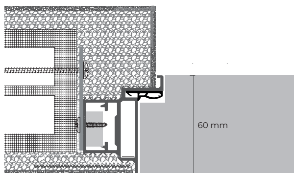
60 mm - a tirare 60 mm - pull version
