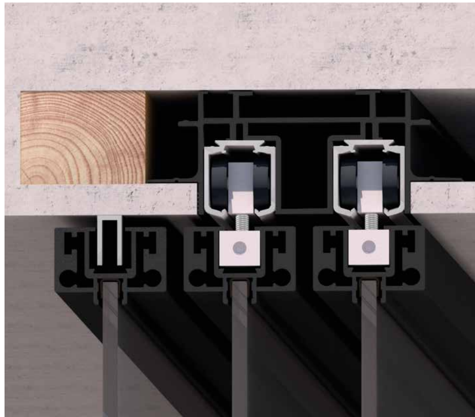
VOLTA 3W2R / 3 ways, 2 rails
