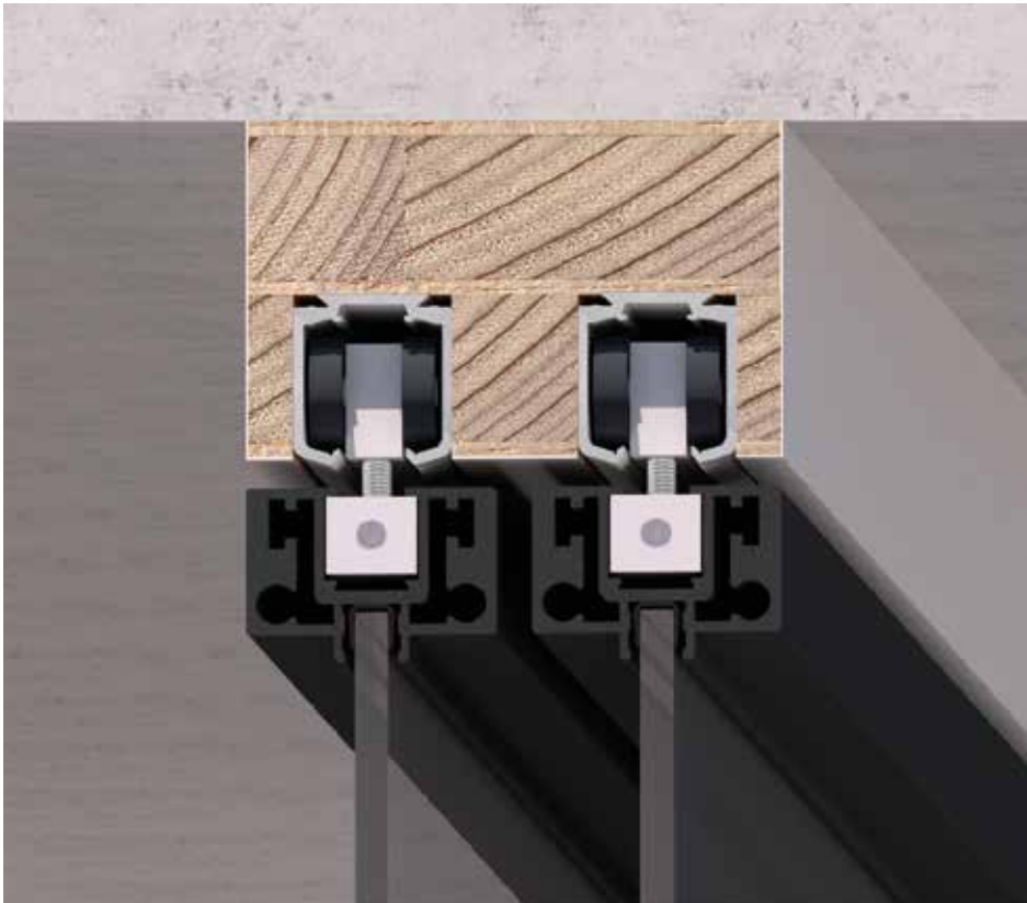
VOLTA M2W2R / 2 ways, 2 rails
