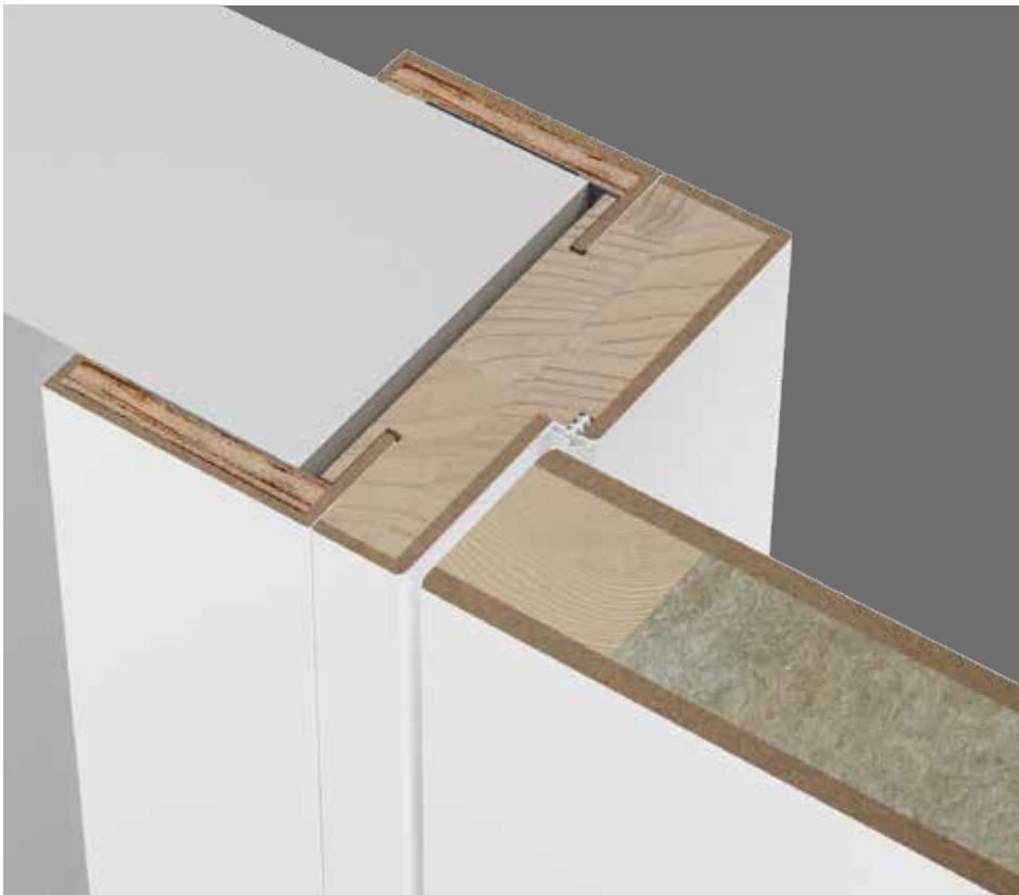
FN / flush on the pull side
