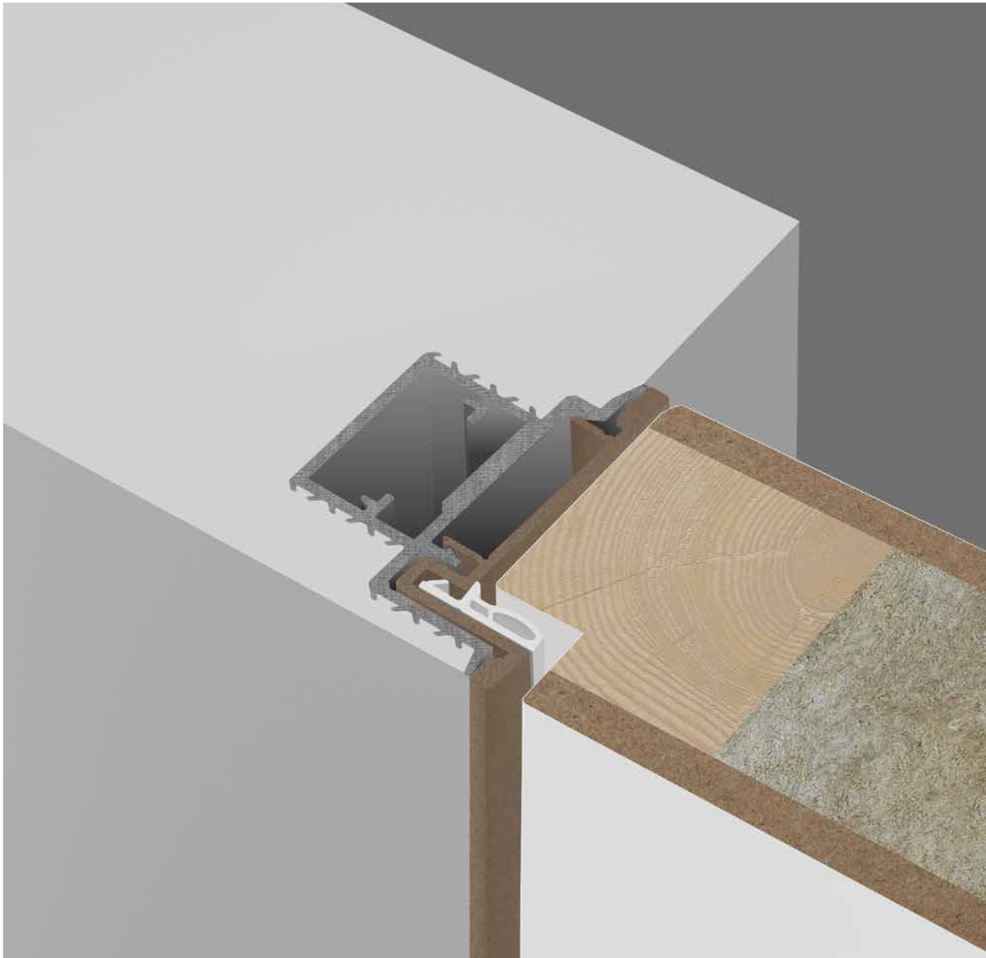
SECRET TWIN PATENTED / Metal cover, flush on the push side
