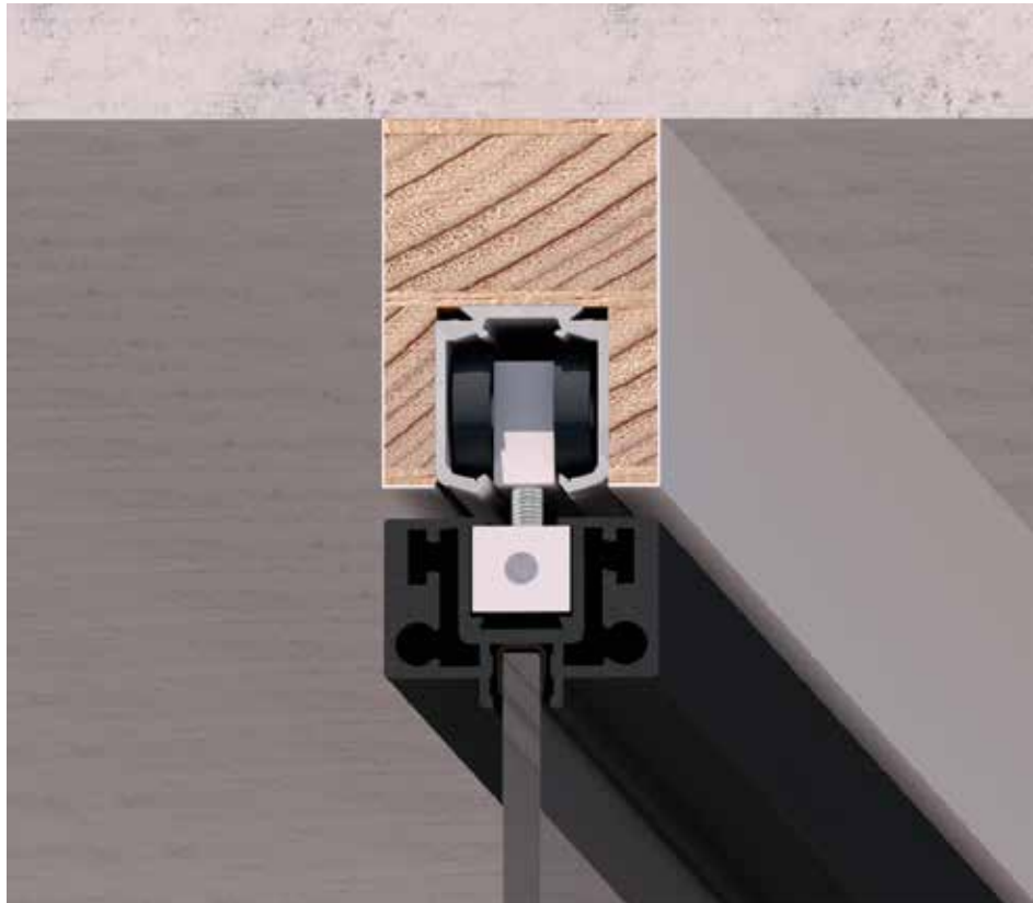
VOLTA M1W1R / 1 way, 1 rail
