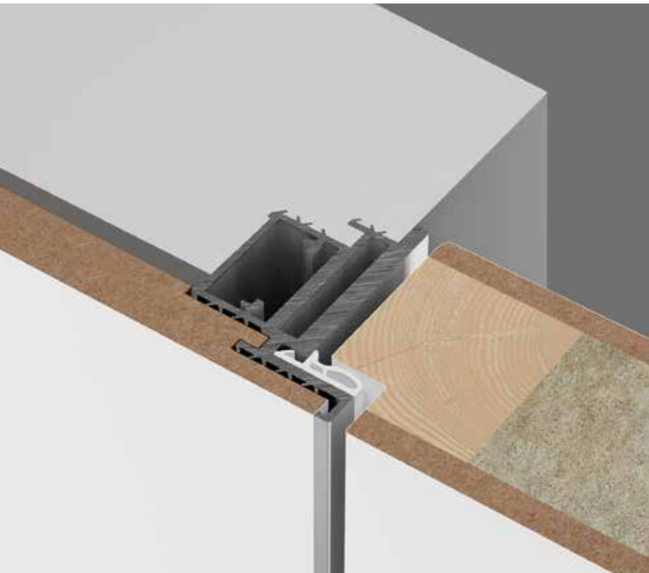
TECNOSECRET / integrated wall paneling
