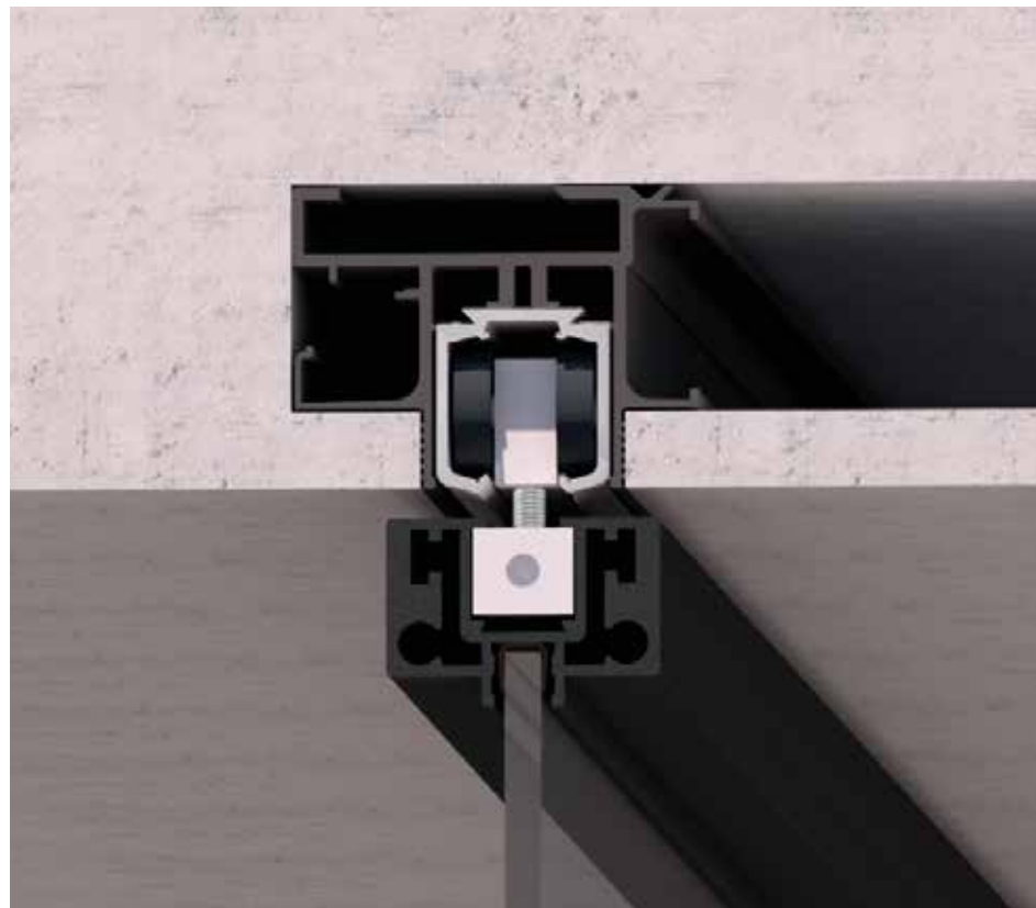
VOLTA 1W1R / 1 way, 1 rail
