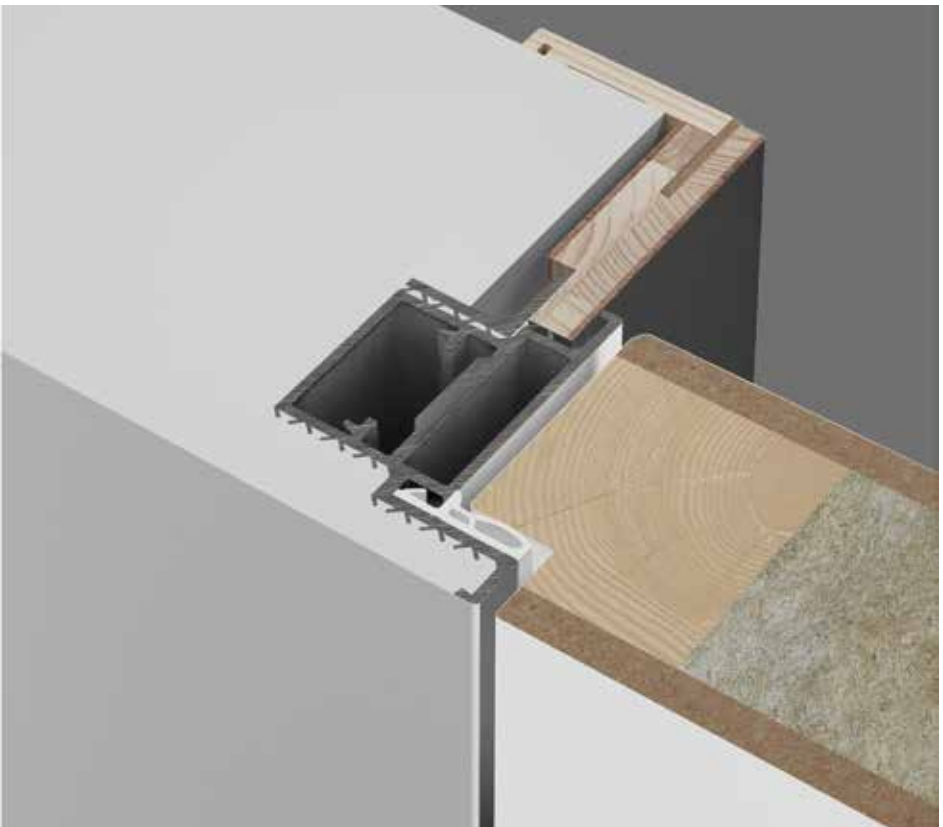
SECRET + SPACER / with spacer and architraves
