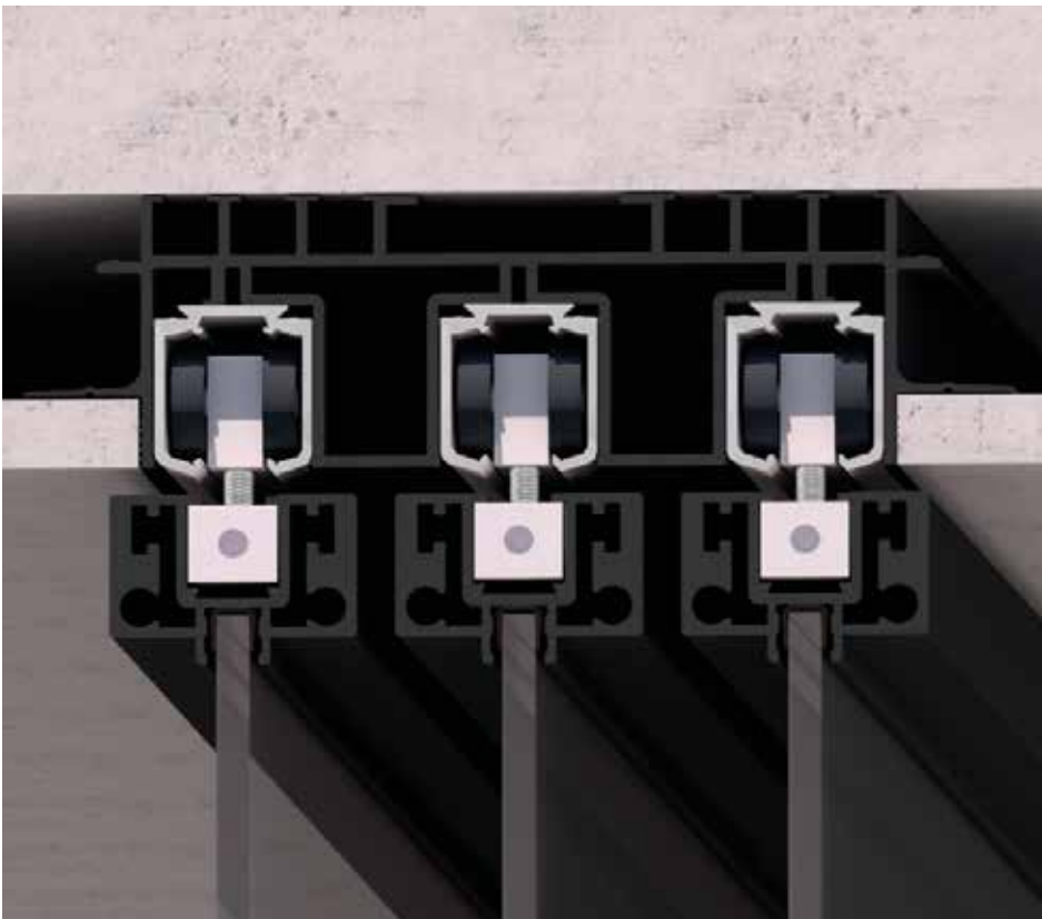
VOLTA 3W3R / 3 ways, 3 rails
