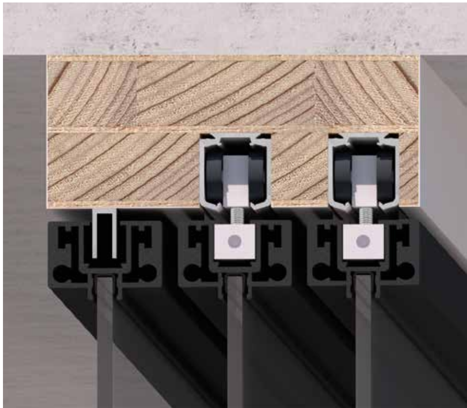
VOLTA M3W2RA / 3 ways, 2 rails
