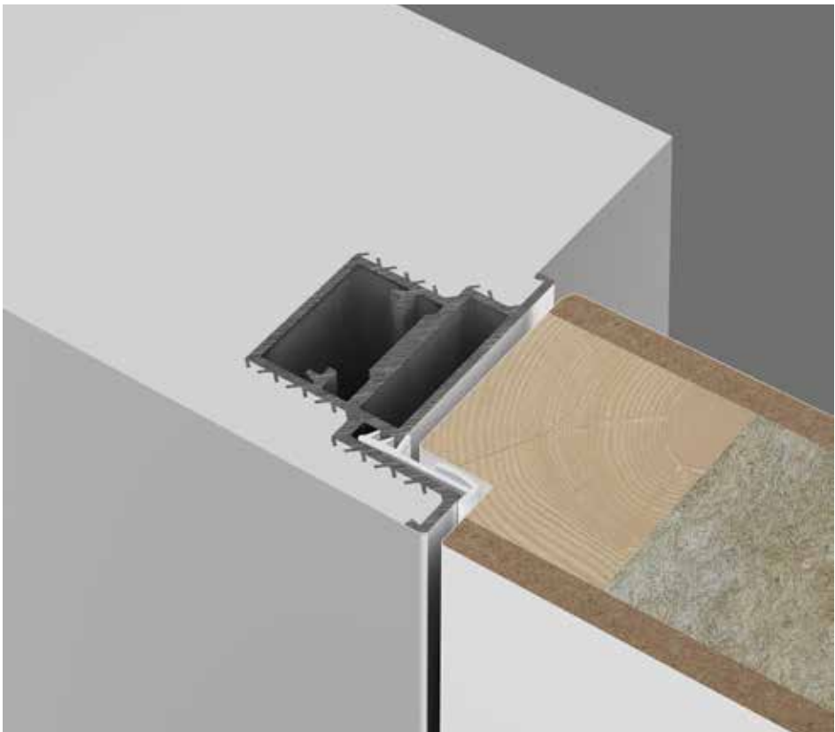
SECRET / flush on the push side
