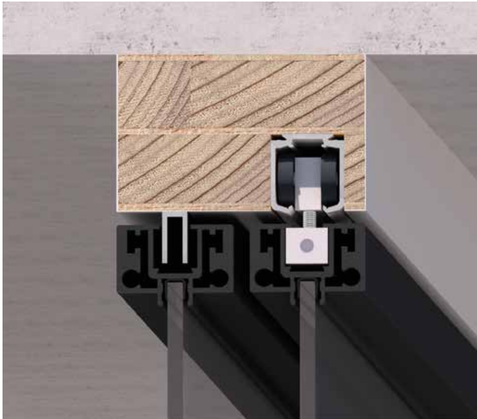
VOLTA M2W1R / 2 ways, 1 rail
