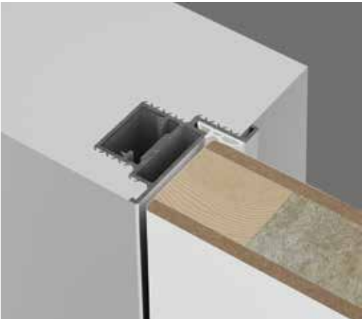
SECRET / flush on the pull side 45 mm
