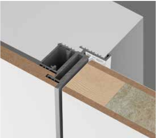
TECNOSECRET / integrated wall paneling, flush on the pull side 45 mm
